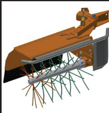
Sucker Remover (SRV)
